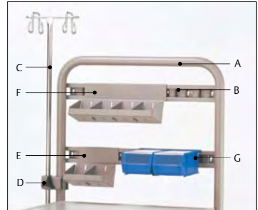
SXSOB Overbridge Assembly (shown with optional accessories)
